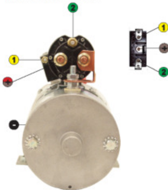
Pr319 Bucher Pump to PS525 Toggle Switch
