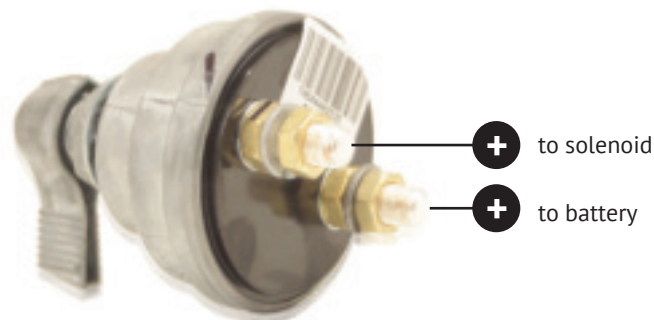
PS025 Safety Cut Off Switch
