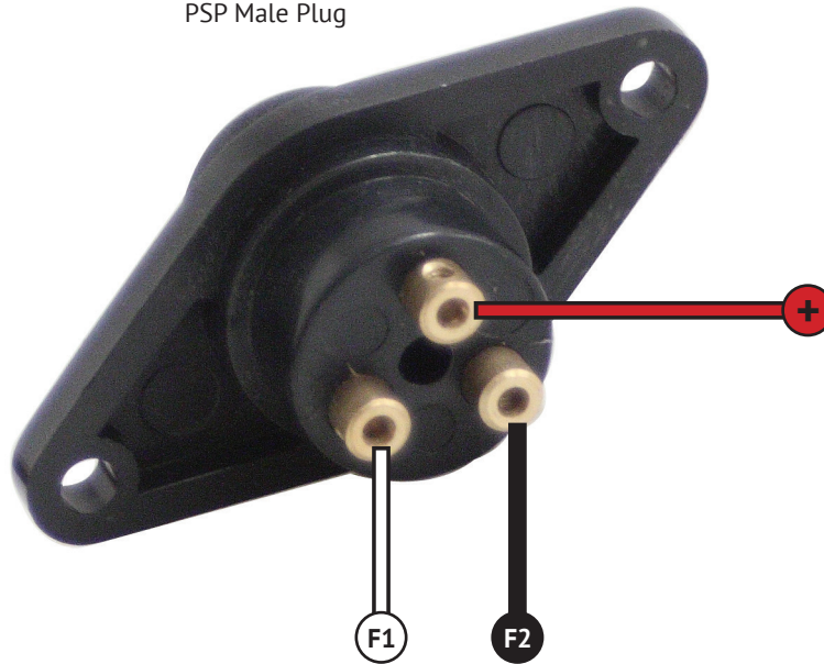
PSP Male Plug
